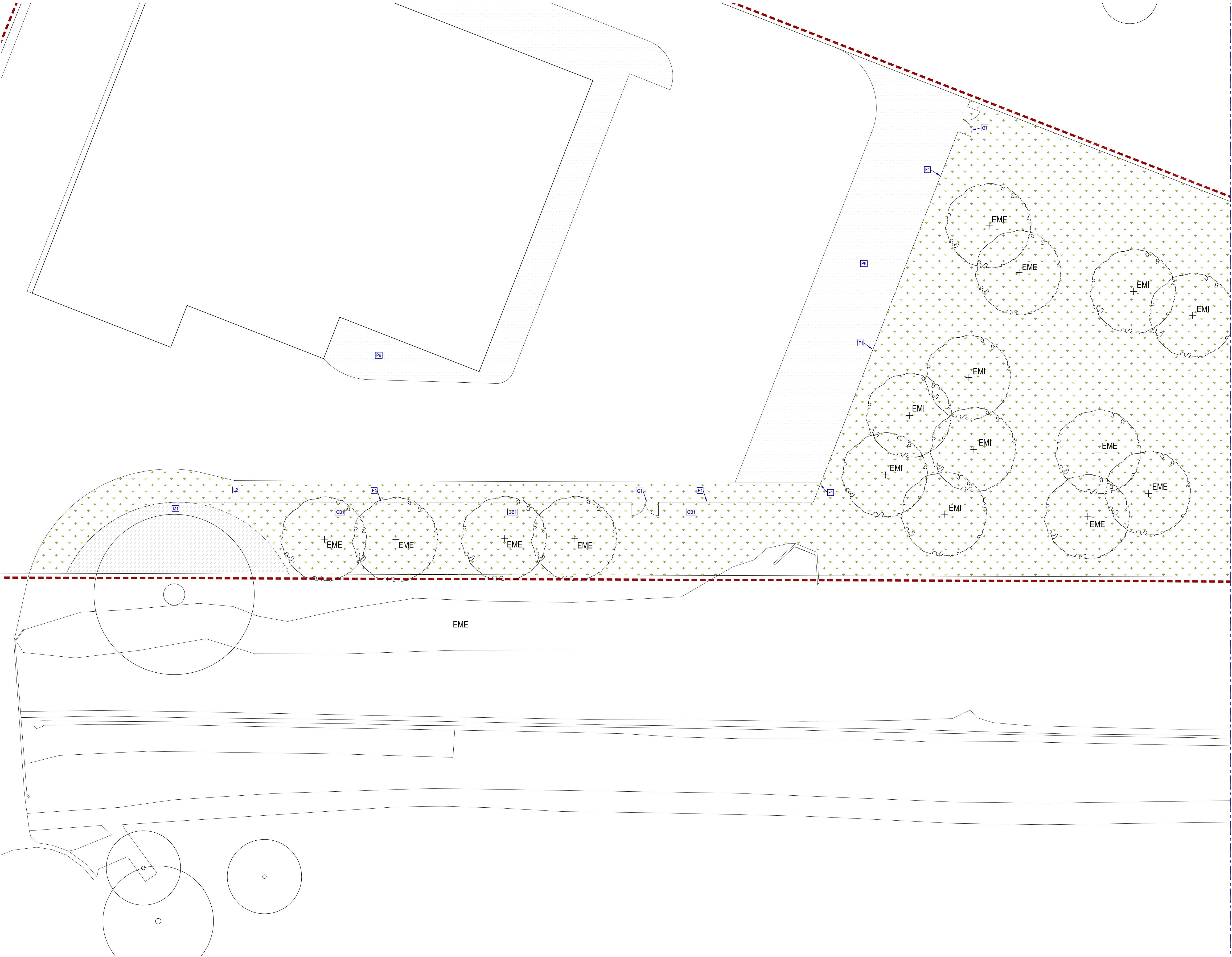
01 SURFACE TREATMENT PLAN 2 202 1:200@A1
